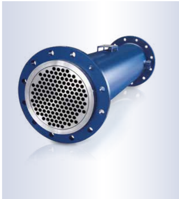
The air-to-water aftercooler is ideal for heat recovery. Designed to provide maximum heat transfer to cooling water when needed
