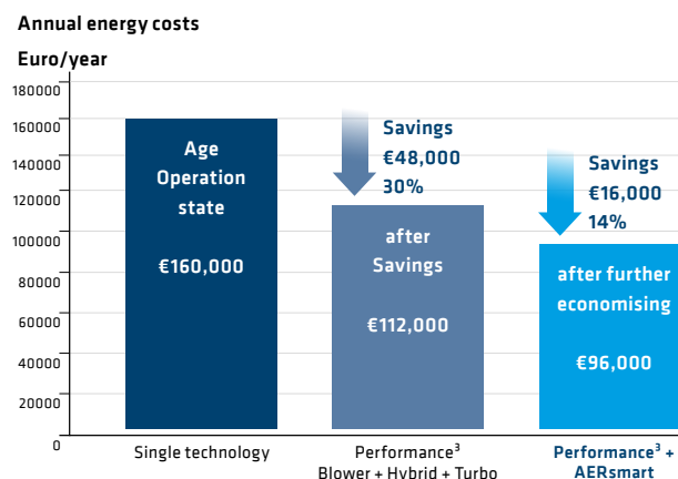
Example of the German wastewater treatment plant with 326,000 population equivalents (PE)
