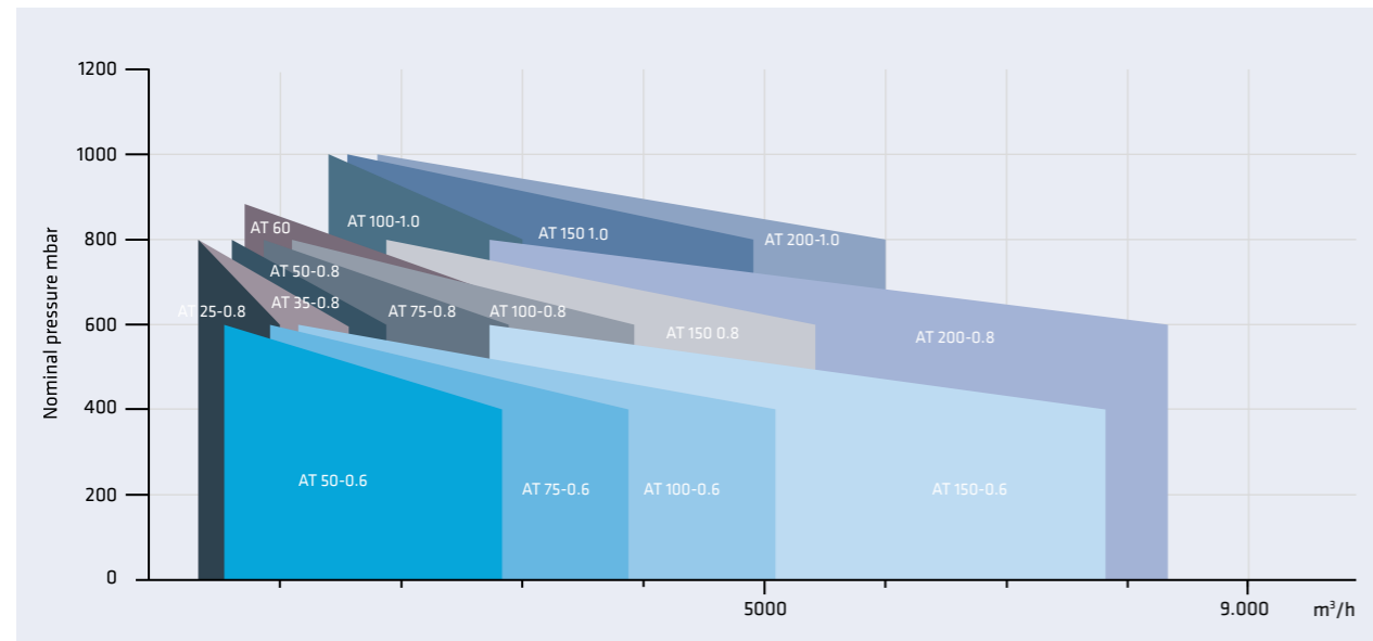
Pressure and volume flow ranges for Generation 5 plus
