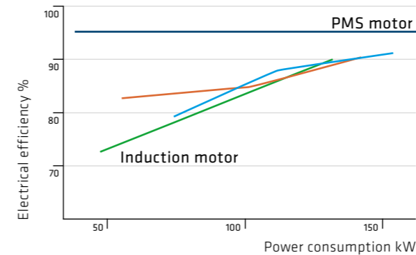
Induction and PMS motor comparison
